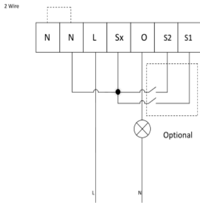
2-wire
