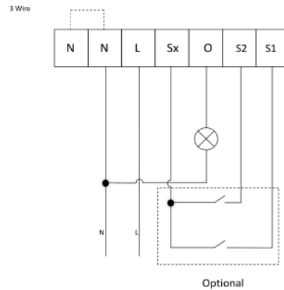
3-wire
